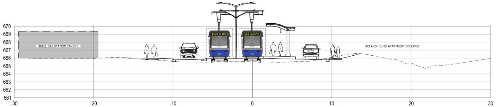
Location B: East platform cross-section, looking east
