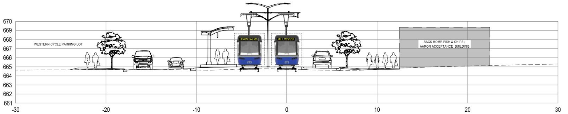
Location A: West platform cross-section, looking east
